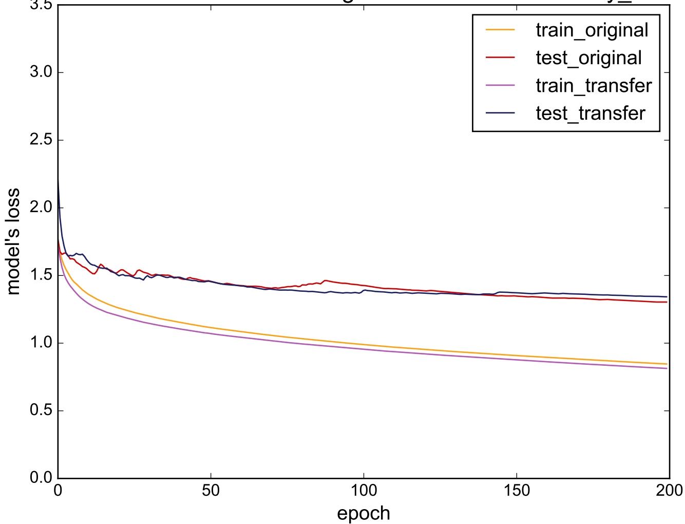
Source: FacesUCR - Target: uWaveGestureLibrary_Y
