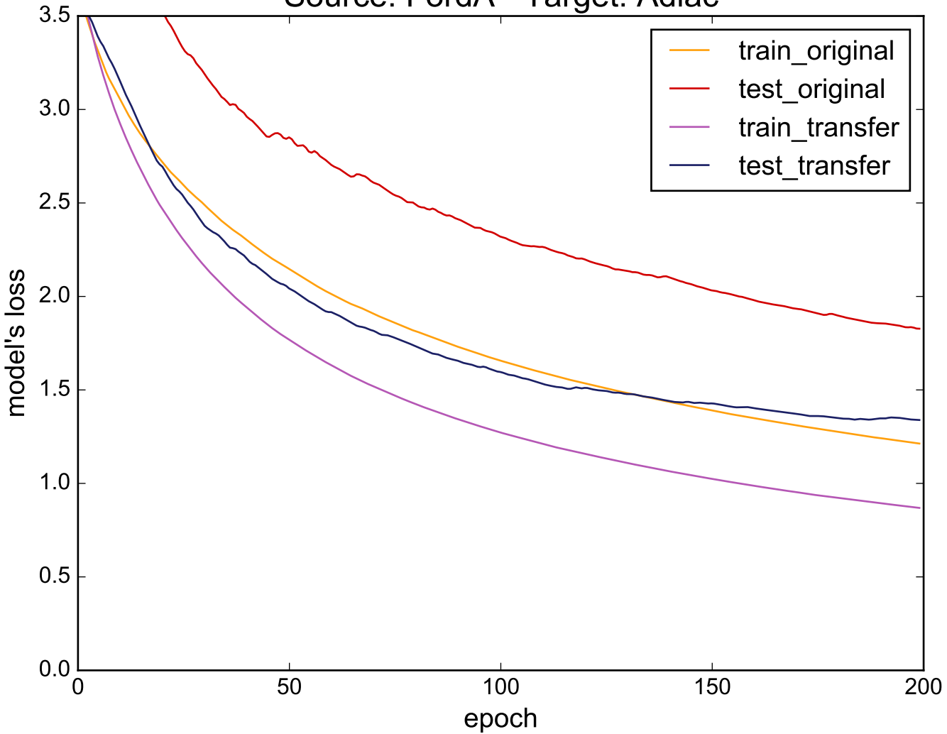
Source: FordA - Target: Adiac
