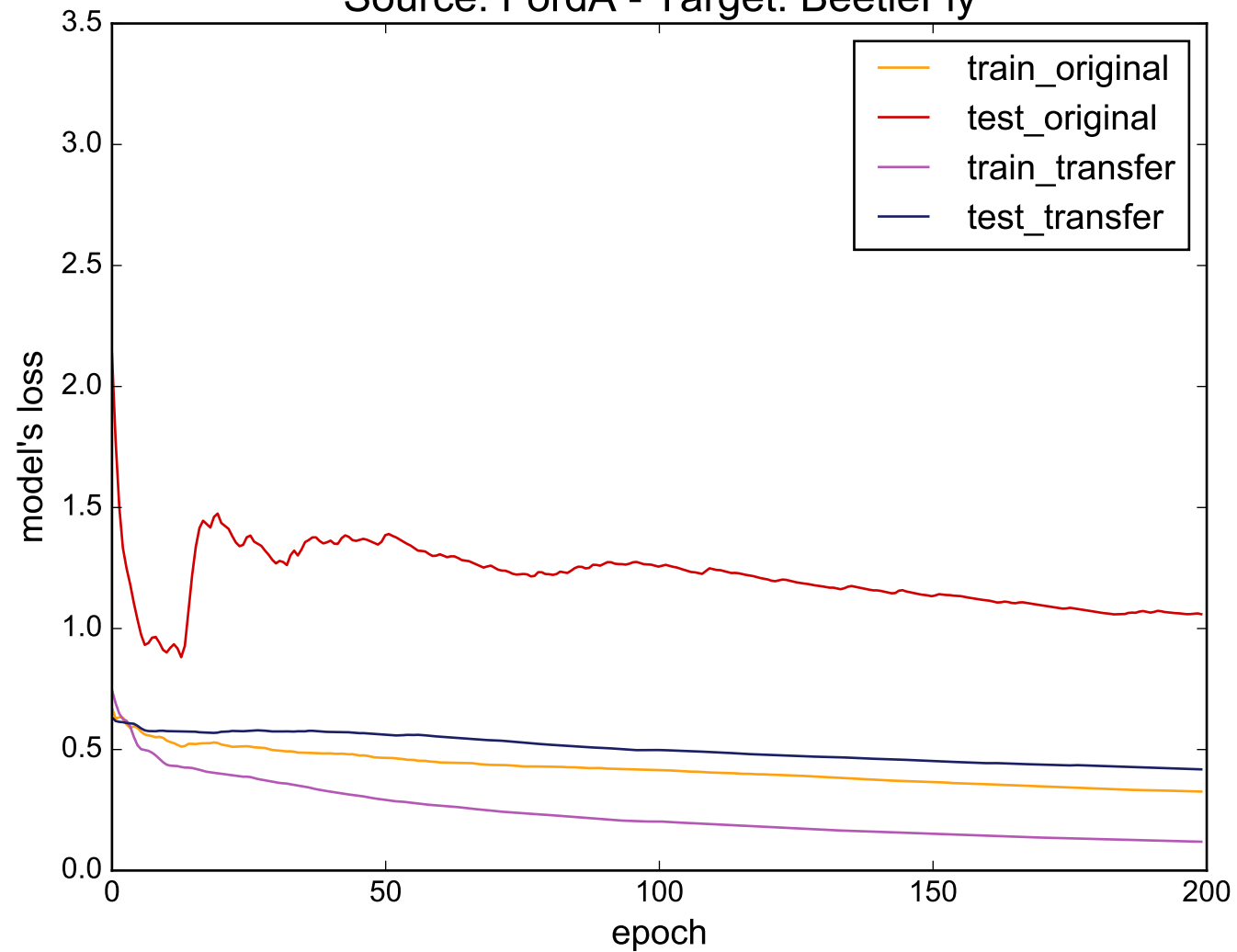
Source: FordA - Target: BeetleFly
