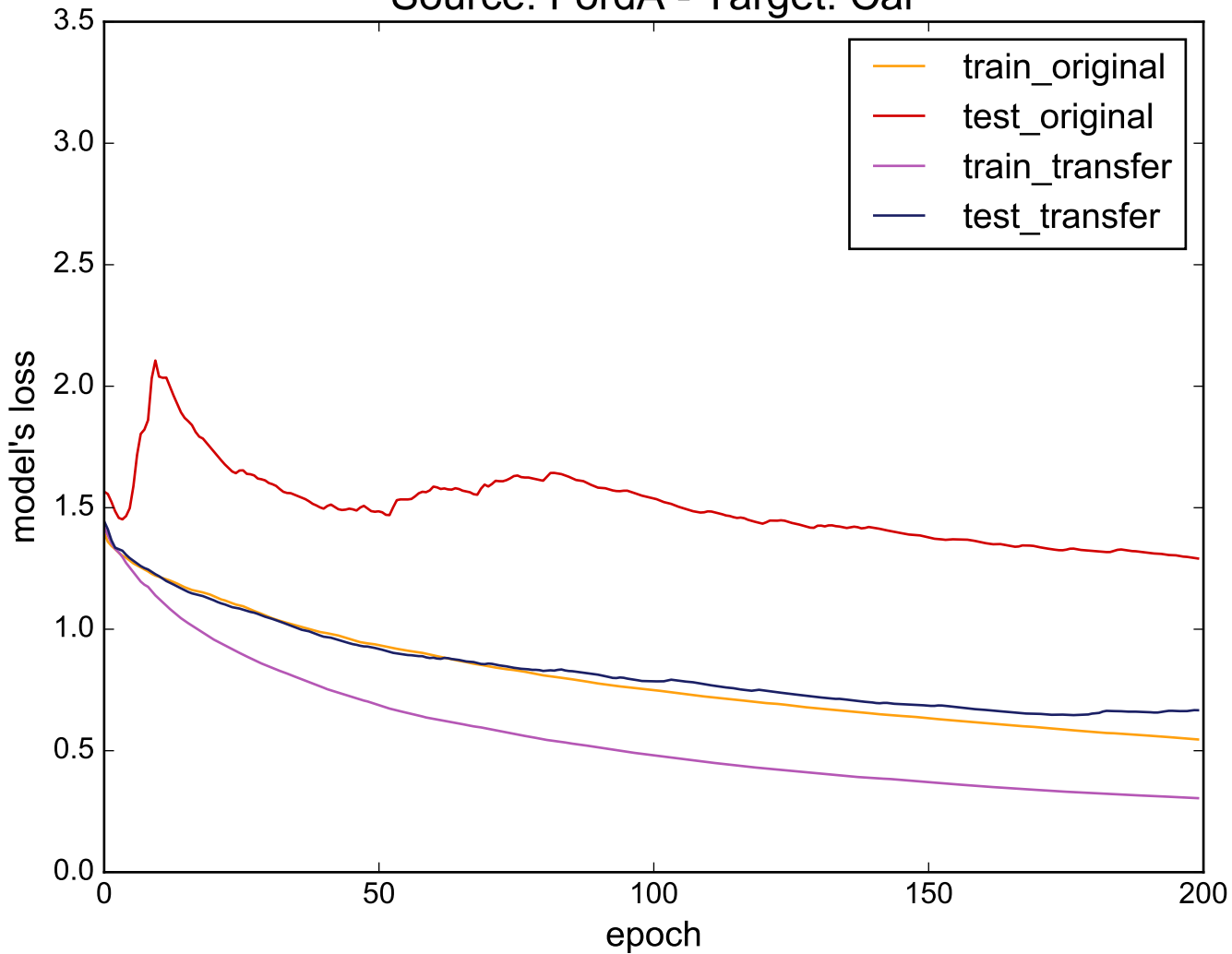
Source: FordA - Target: Car
