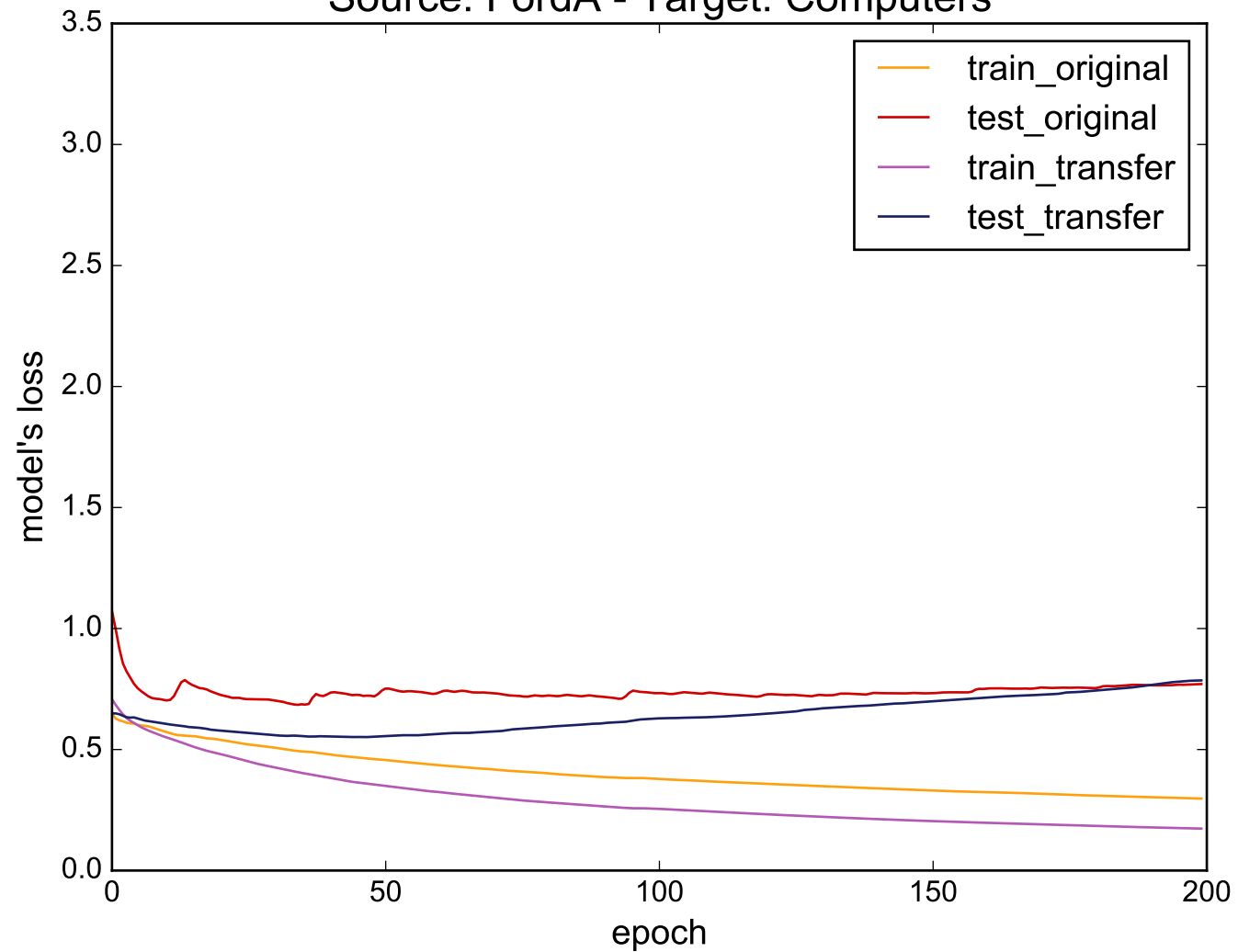
Source: FordA - Target: Computers
