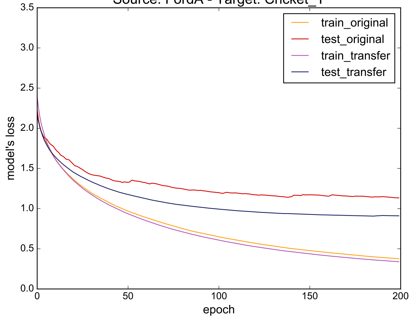
Source: FordA - Target: Cricket_Y
