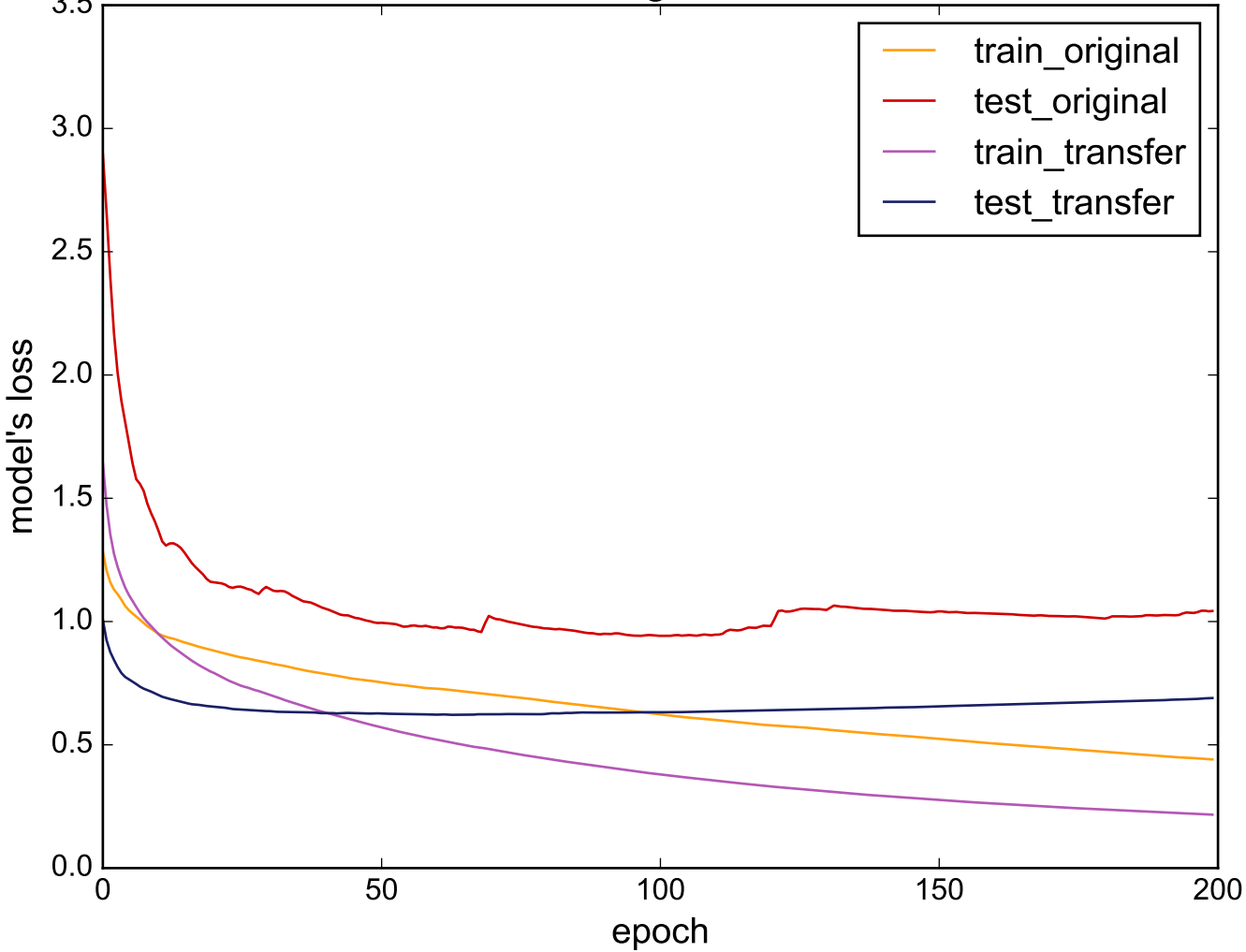
Source: FordA - Target: DistalPhalanxTW
