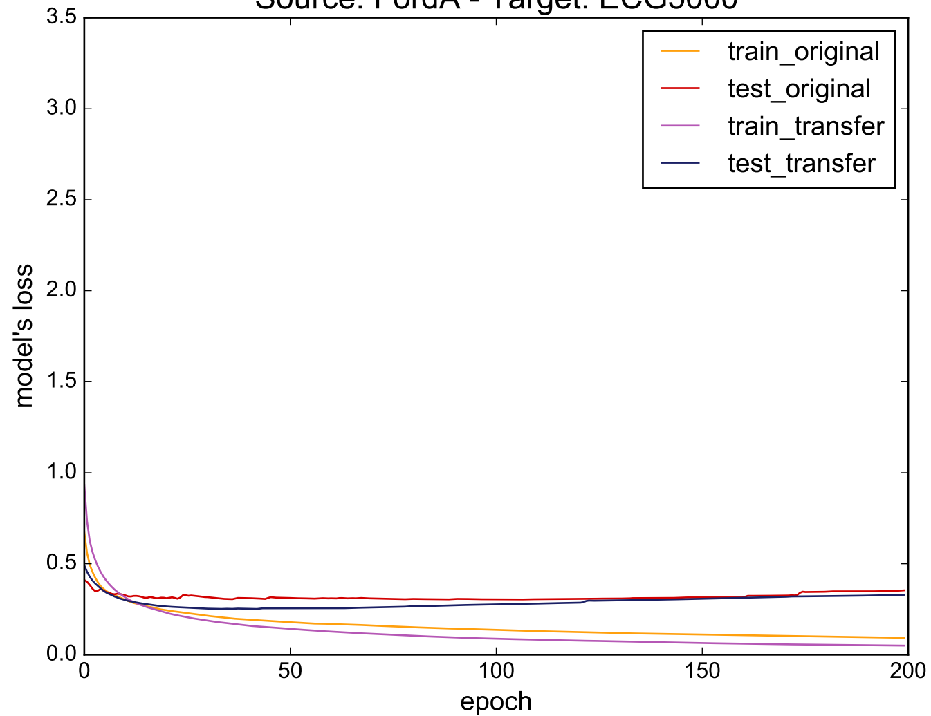
Source: FordA - Target: ECG5000
