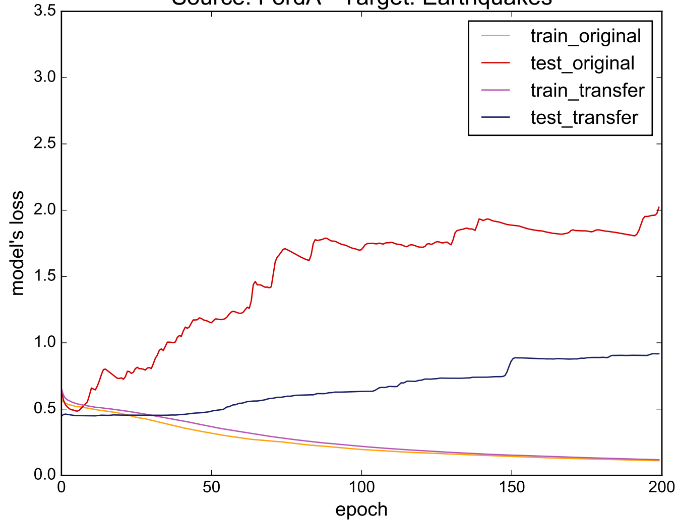
Source: FordA - Target: Earthquakes
