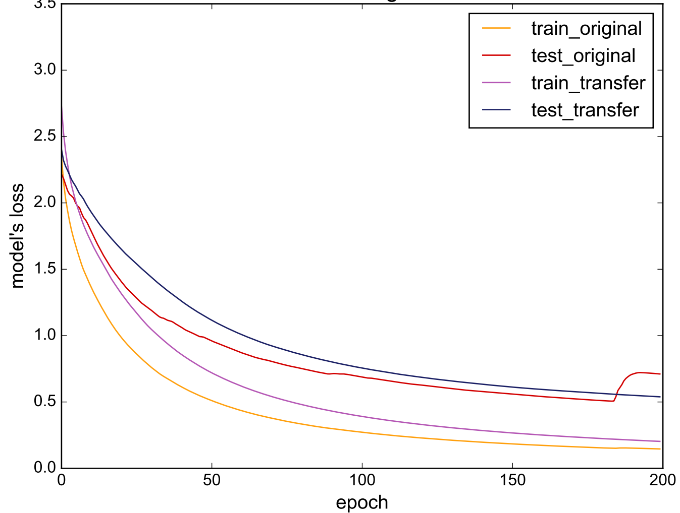
Source: FordA - Target: FacesUCR
