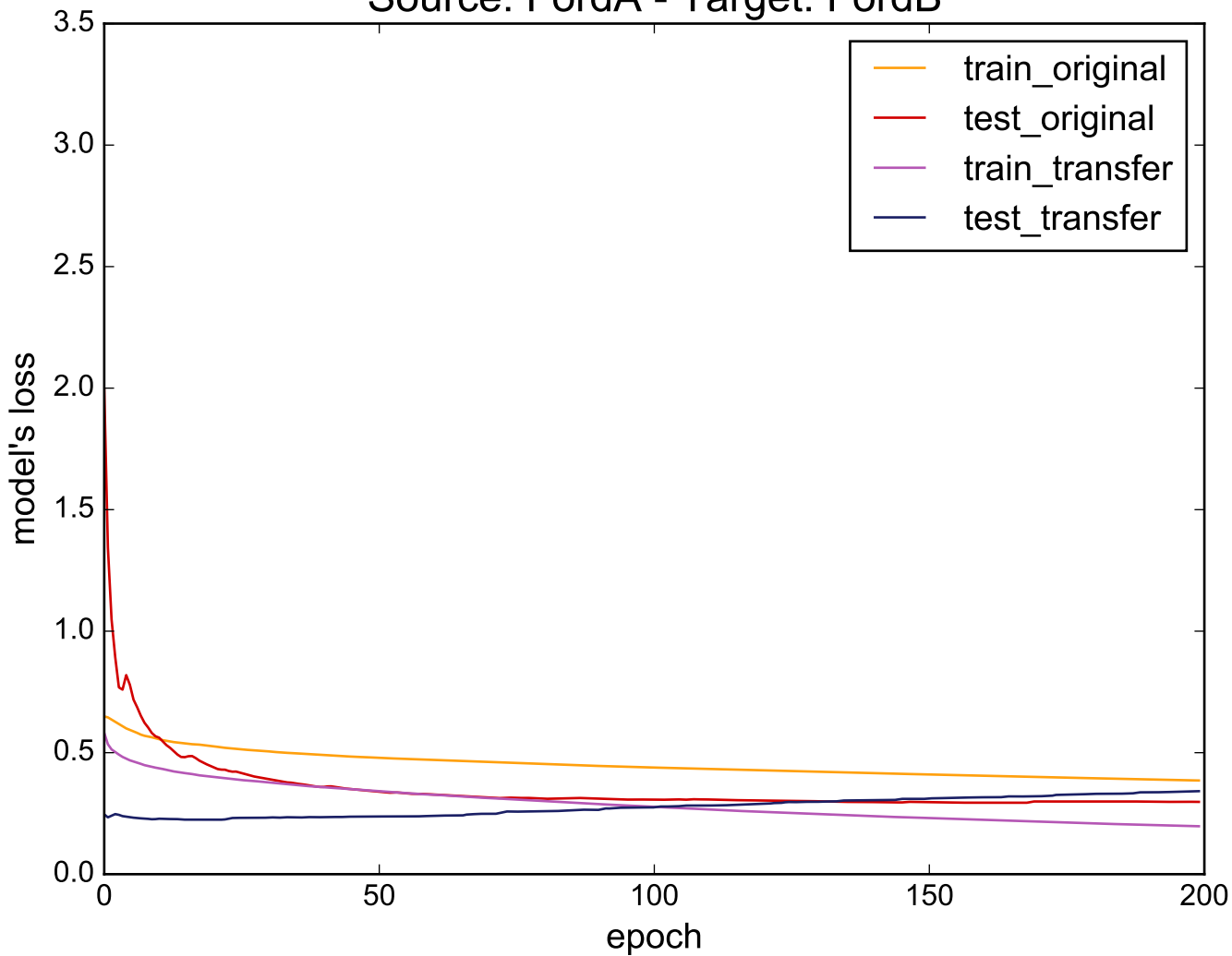
Source: FordA - Target: FordB
