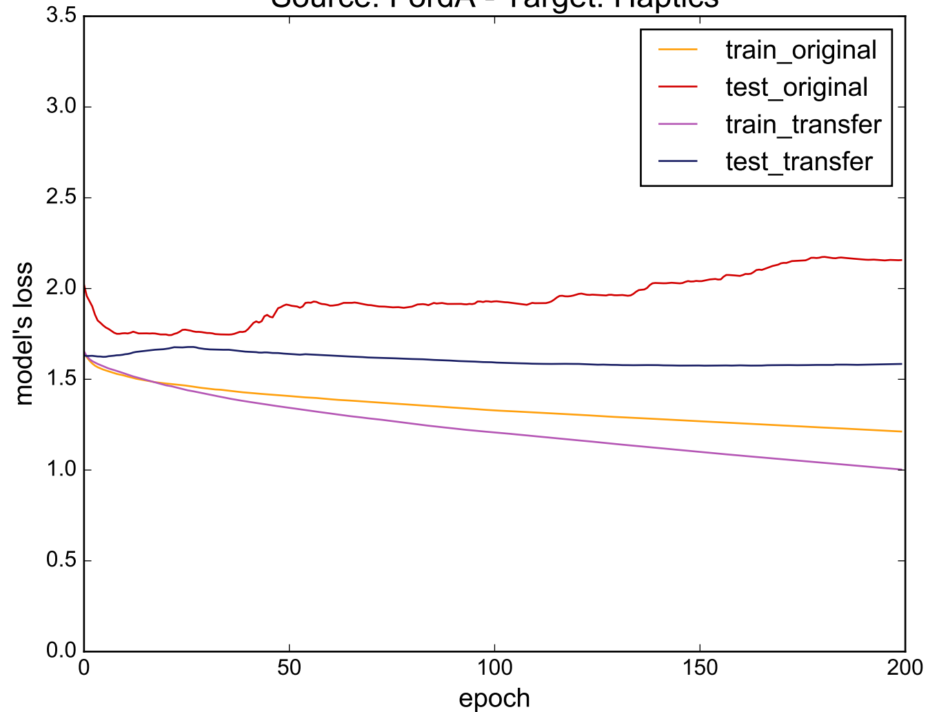
Source: FordA - Target: Haptics
