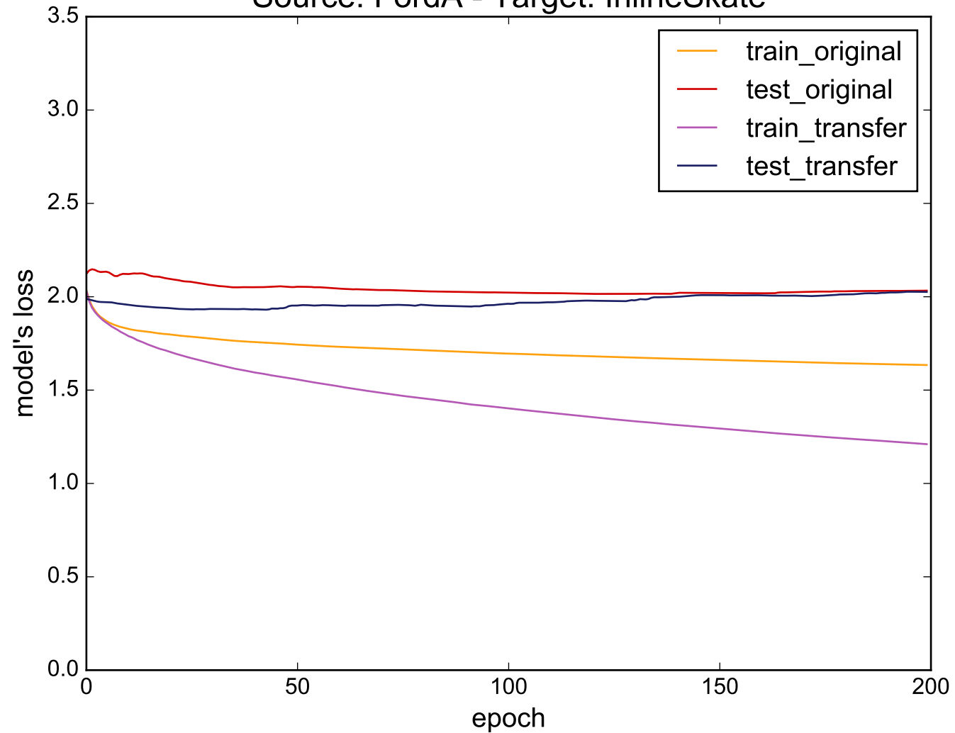
Source: FordA - Target: InlineSkate
