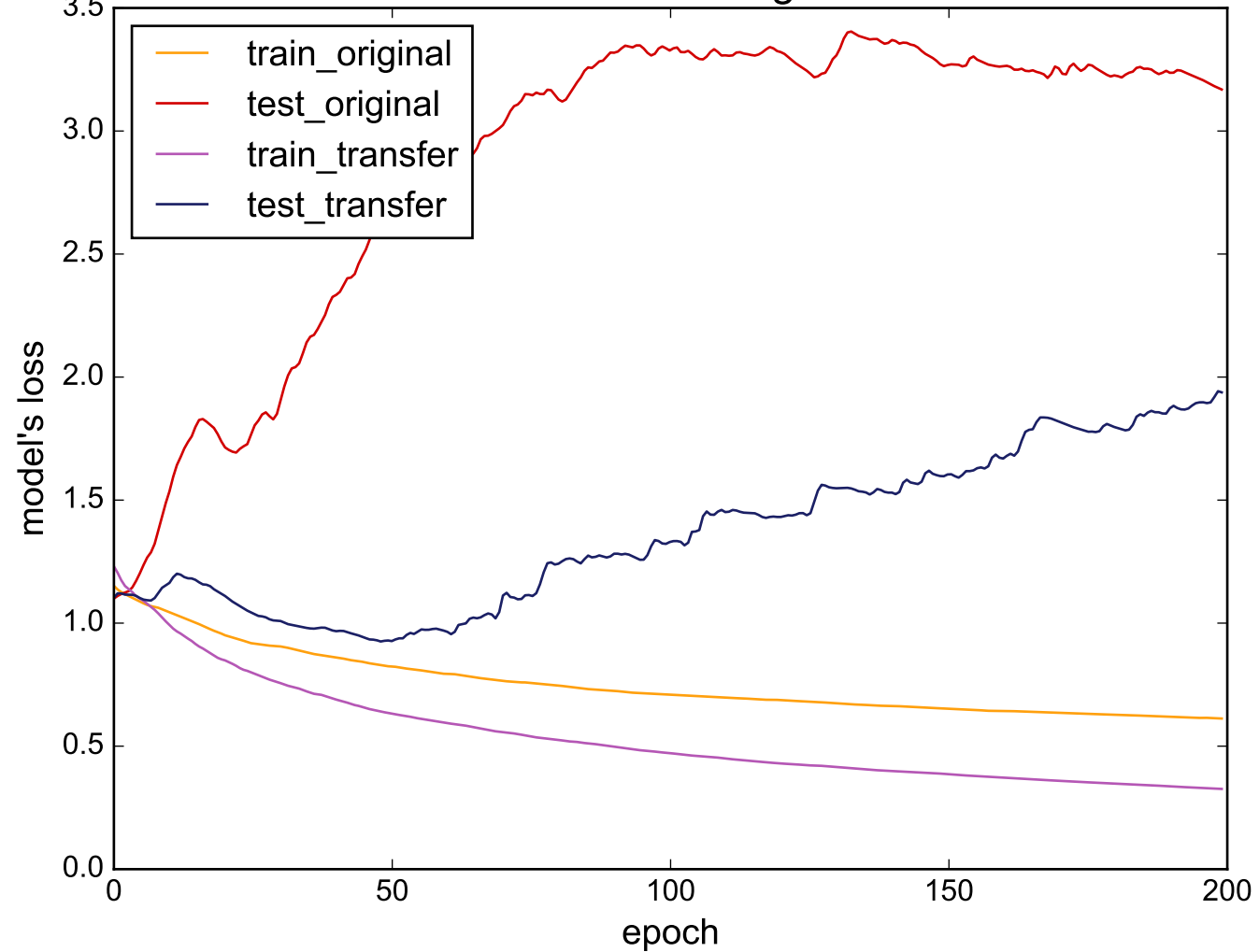
Source: FordA - Target: Meat
