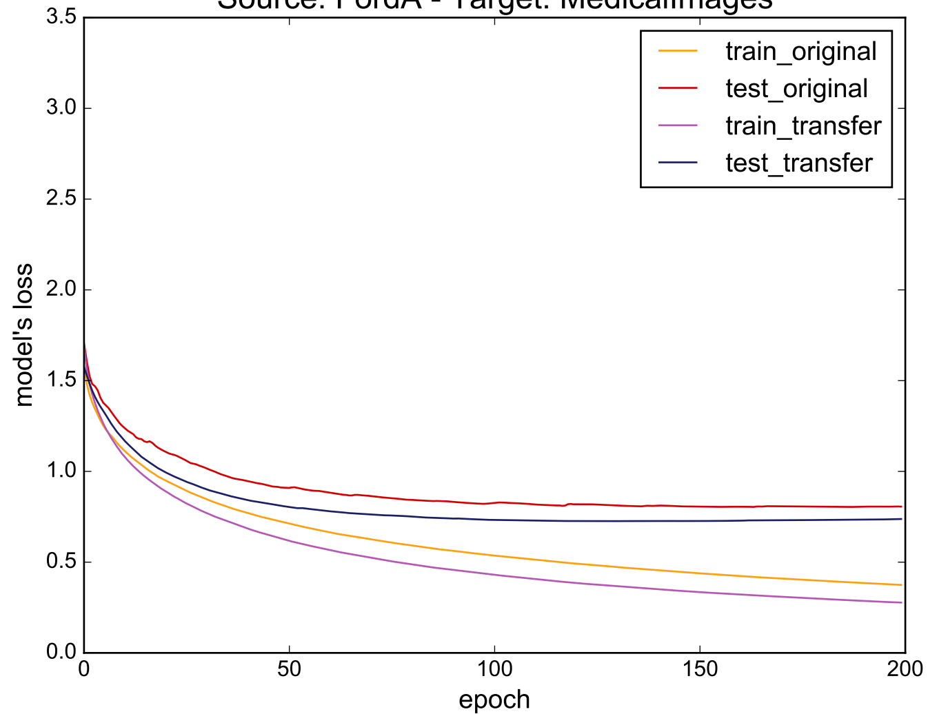
Source: FordA - Target: MedicalImages
