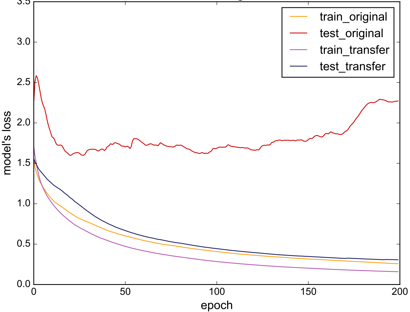
Source: FordA - Target: OSULeaf
