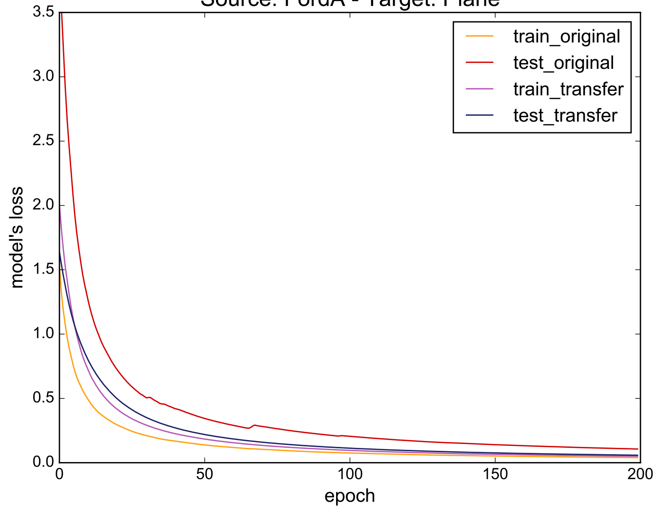
Source: FordA - Target: Plane
