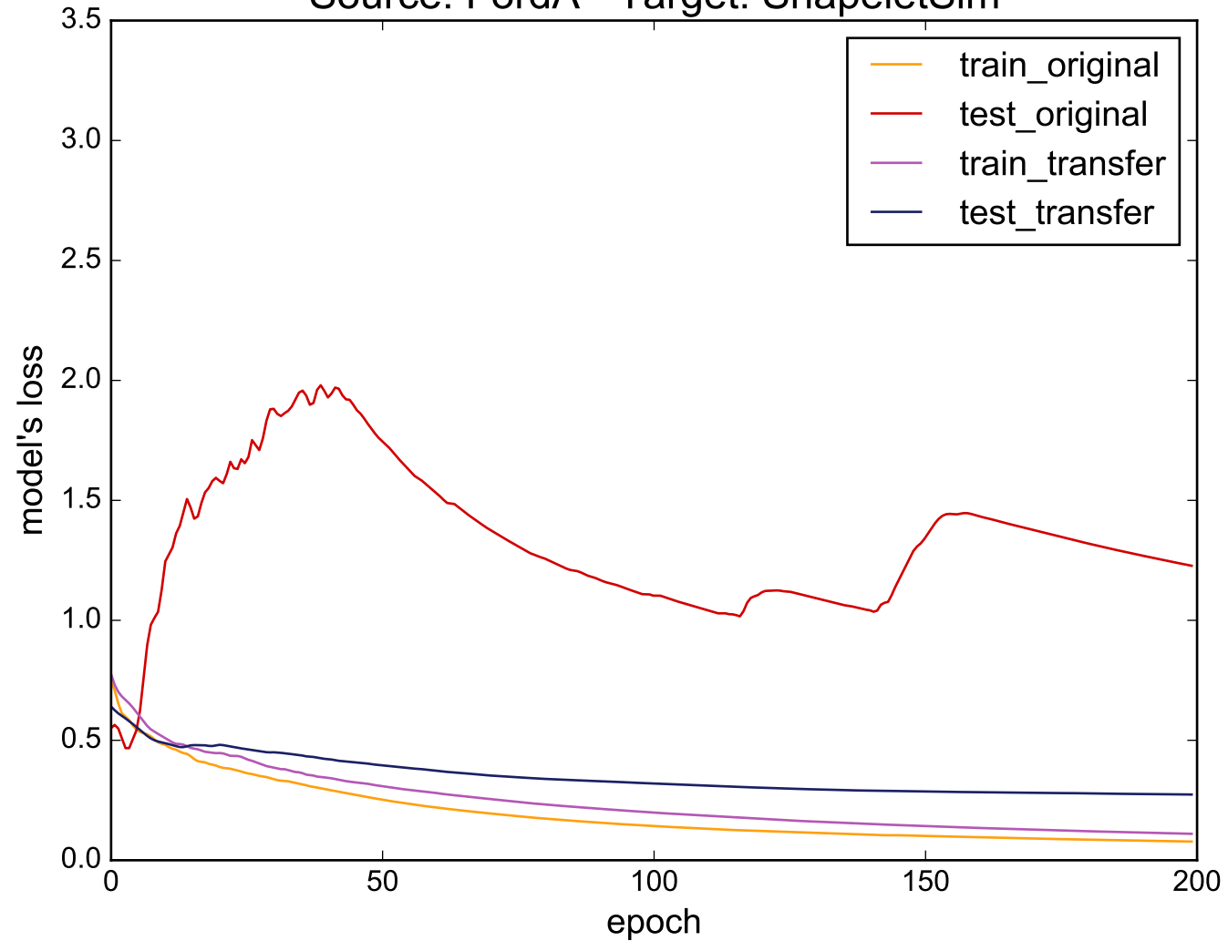
Source: FordA - Target: ShapeletSim
