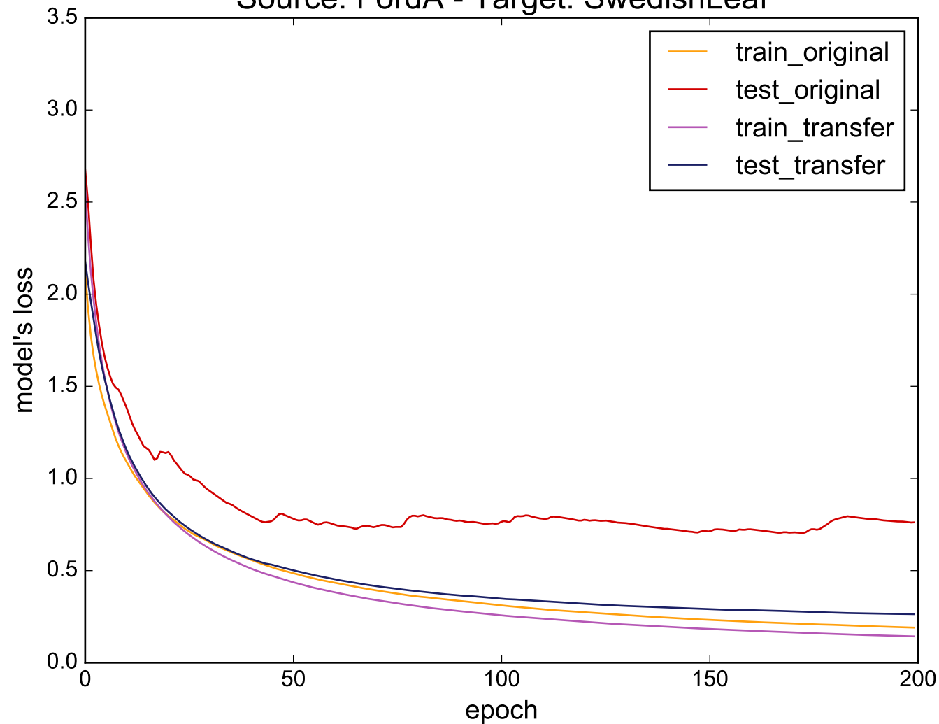
Source: FordA - Target: SwedishLeaf
