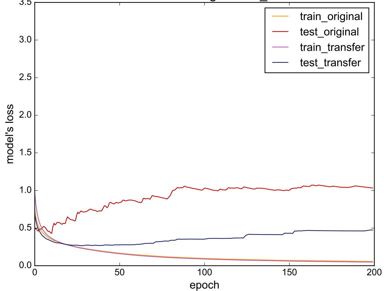
Source: FordA - Target: Two_Patterns
