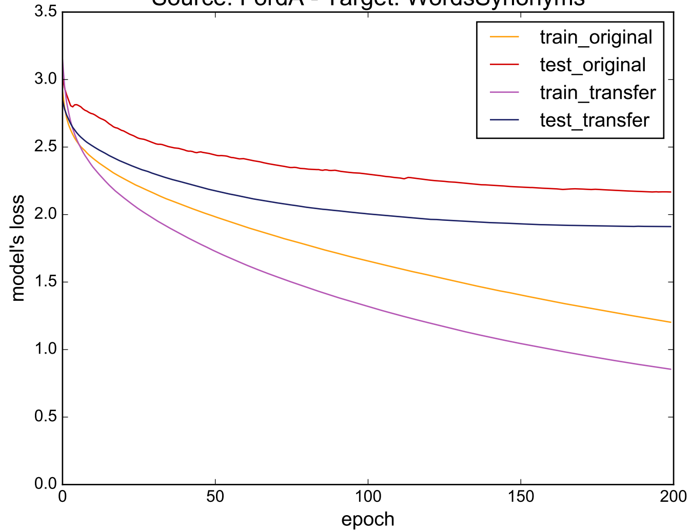
Source: FordA - Target: WordsSynonyms
