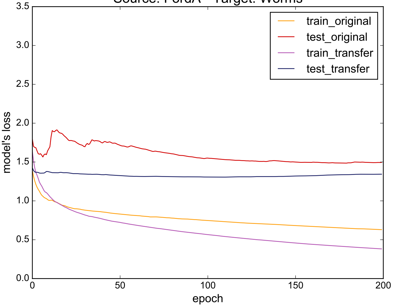
Source: FordA - Target: Worms
