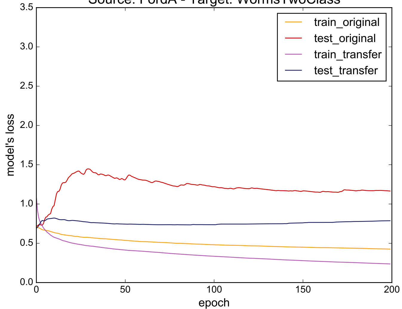
Source: FordA - Target: WormsTwoClass
