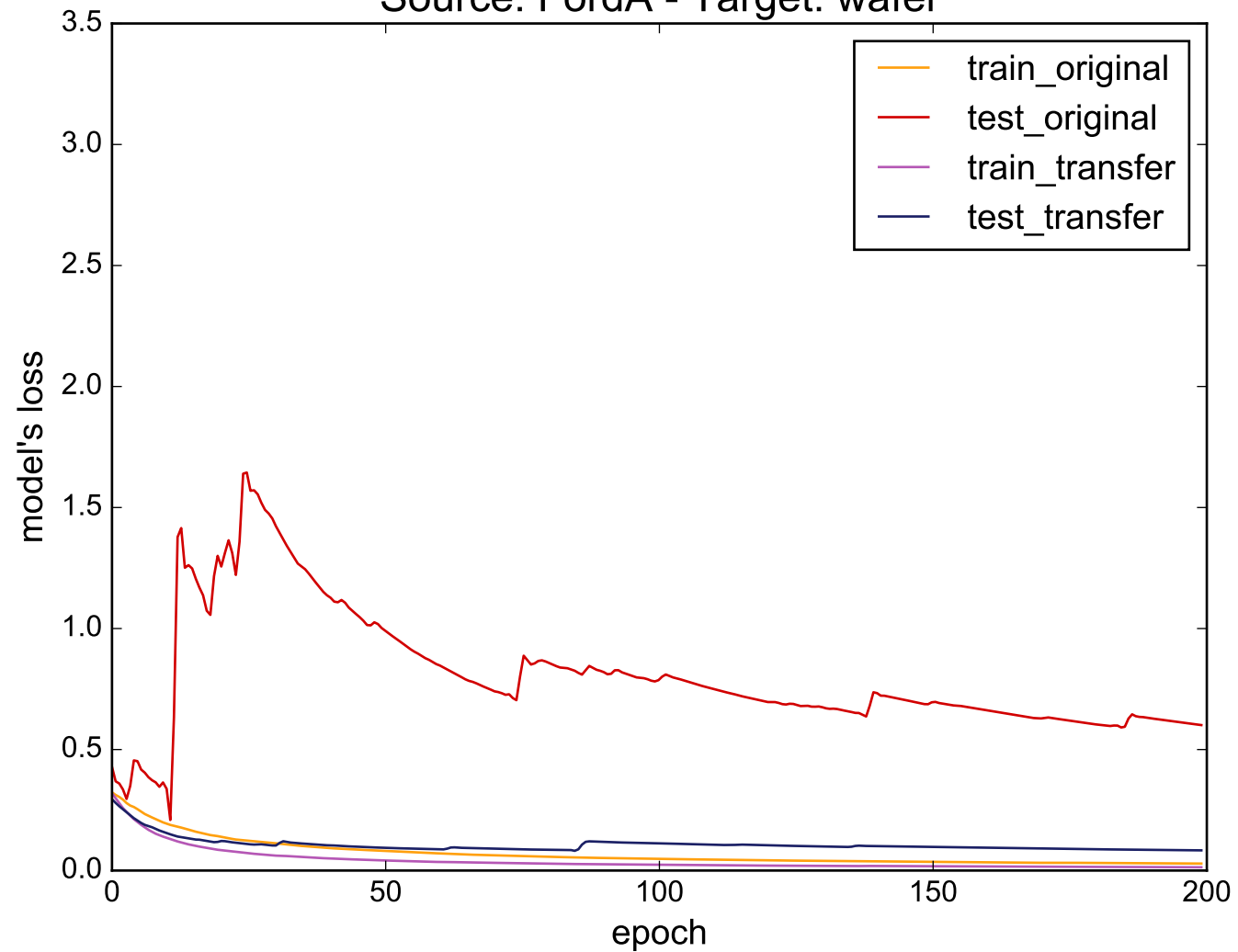
Source: FordA - Target: wafer
