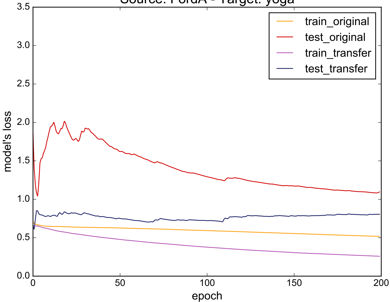
Source: FordA - Target: yoga
