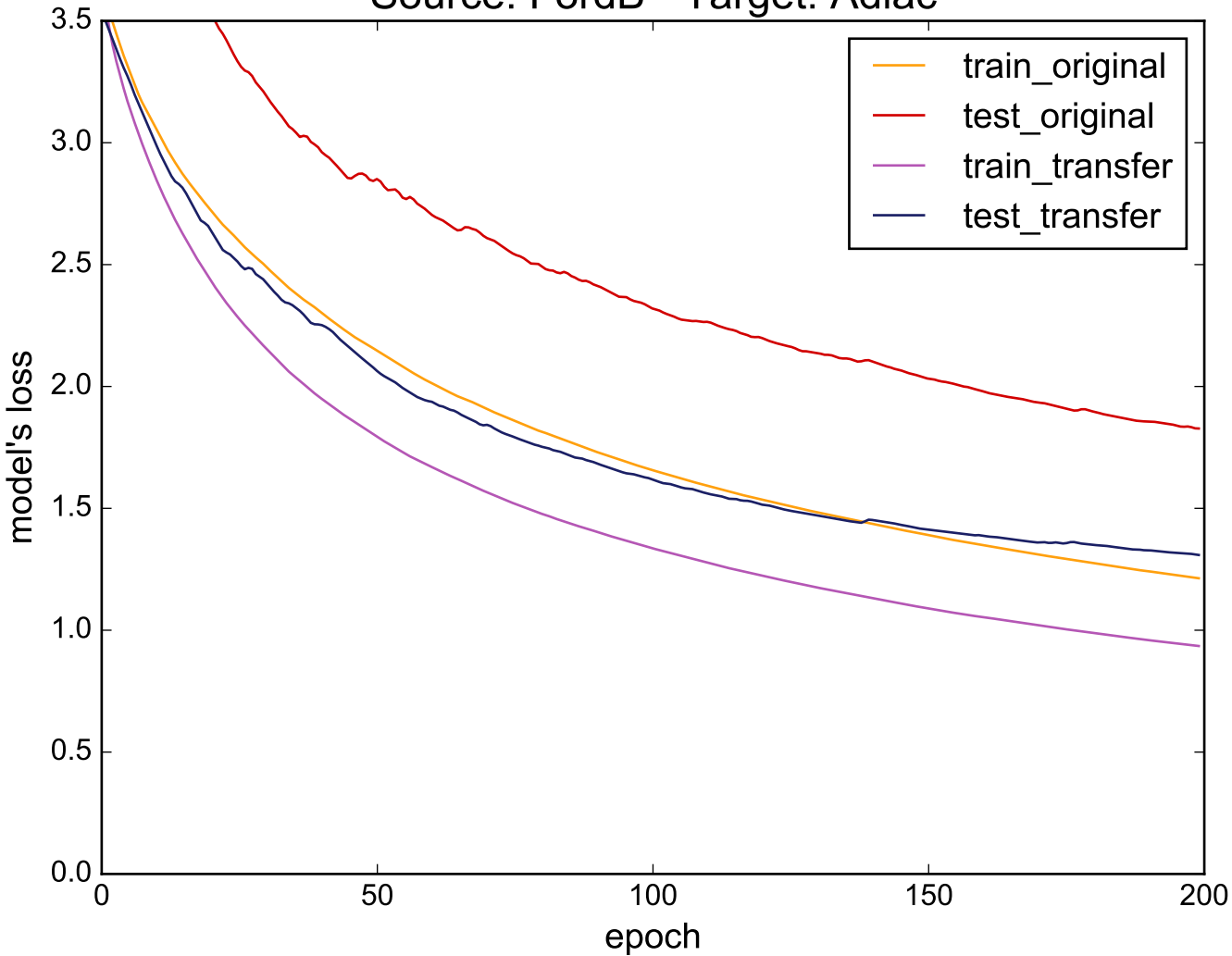
Source: FordB - Target: Adiac
