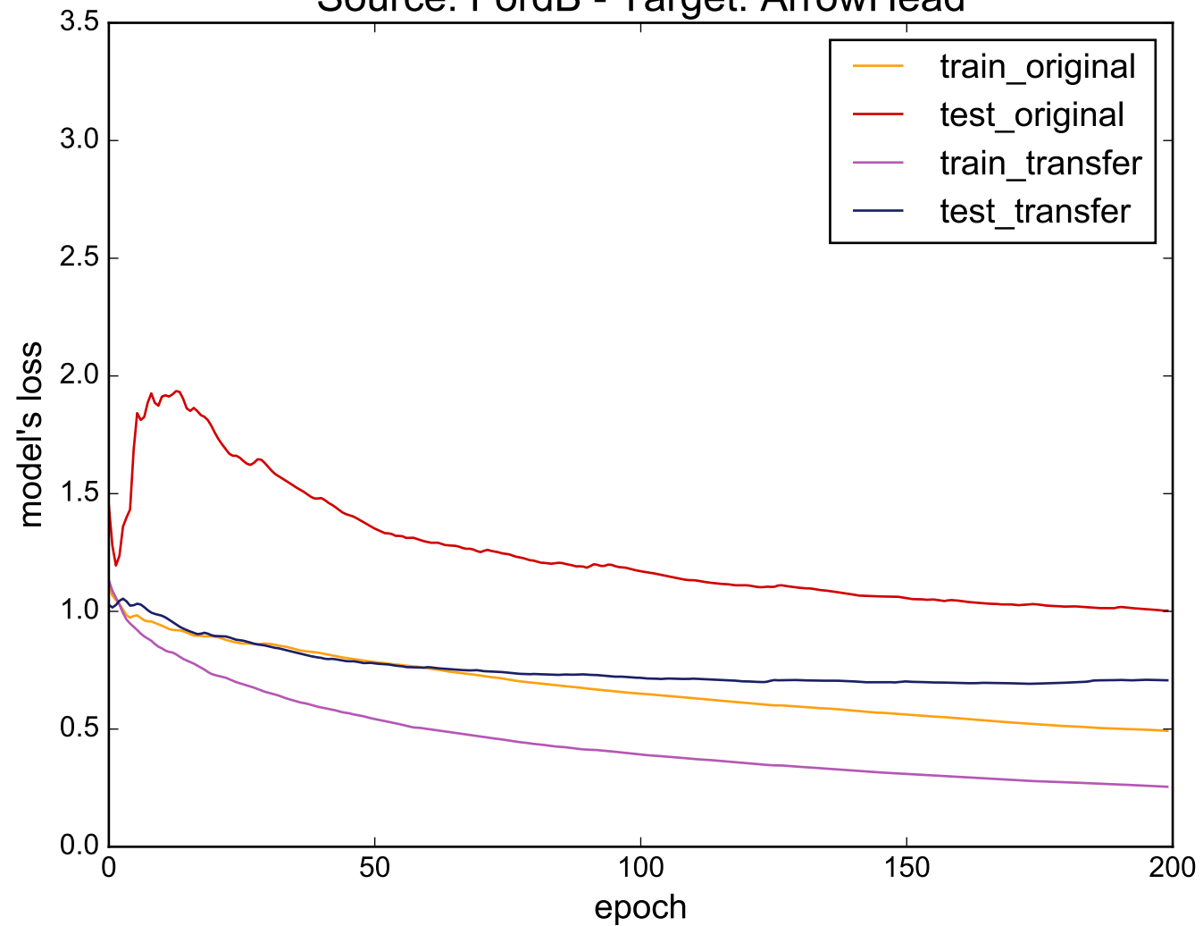
Source: FordB - Target: ArrowHead
