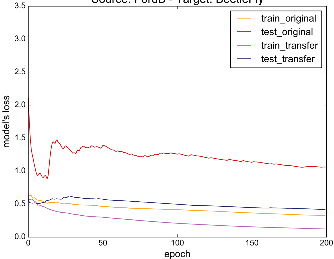
Source: FordB - Target: BeetleFly
