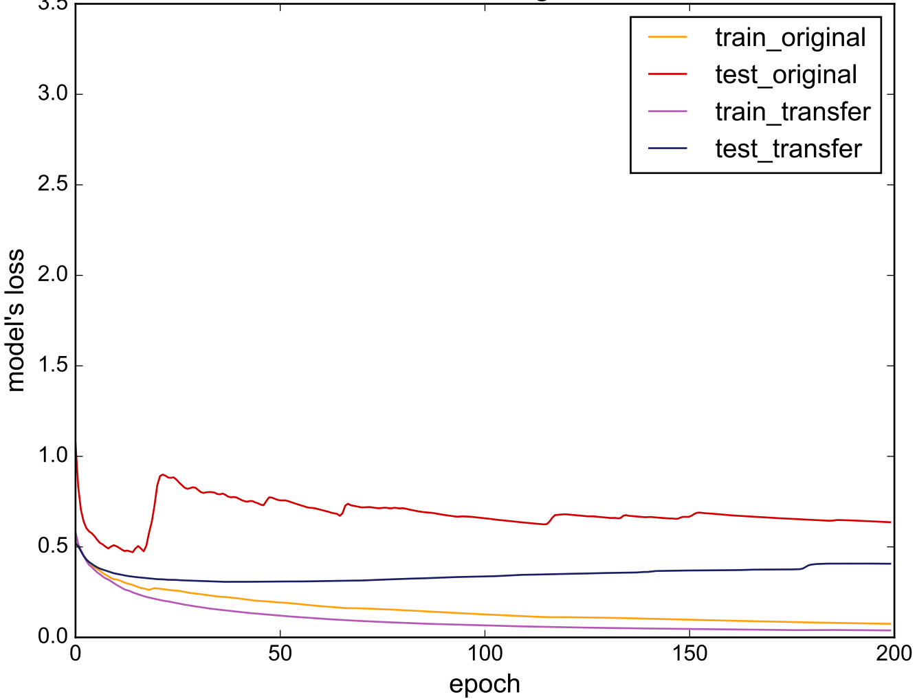
Source: FordB - Target: ECG200
