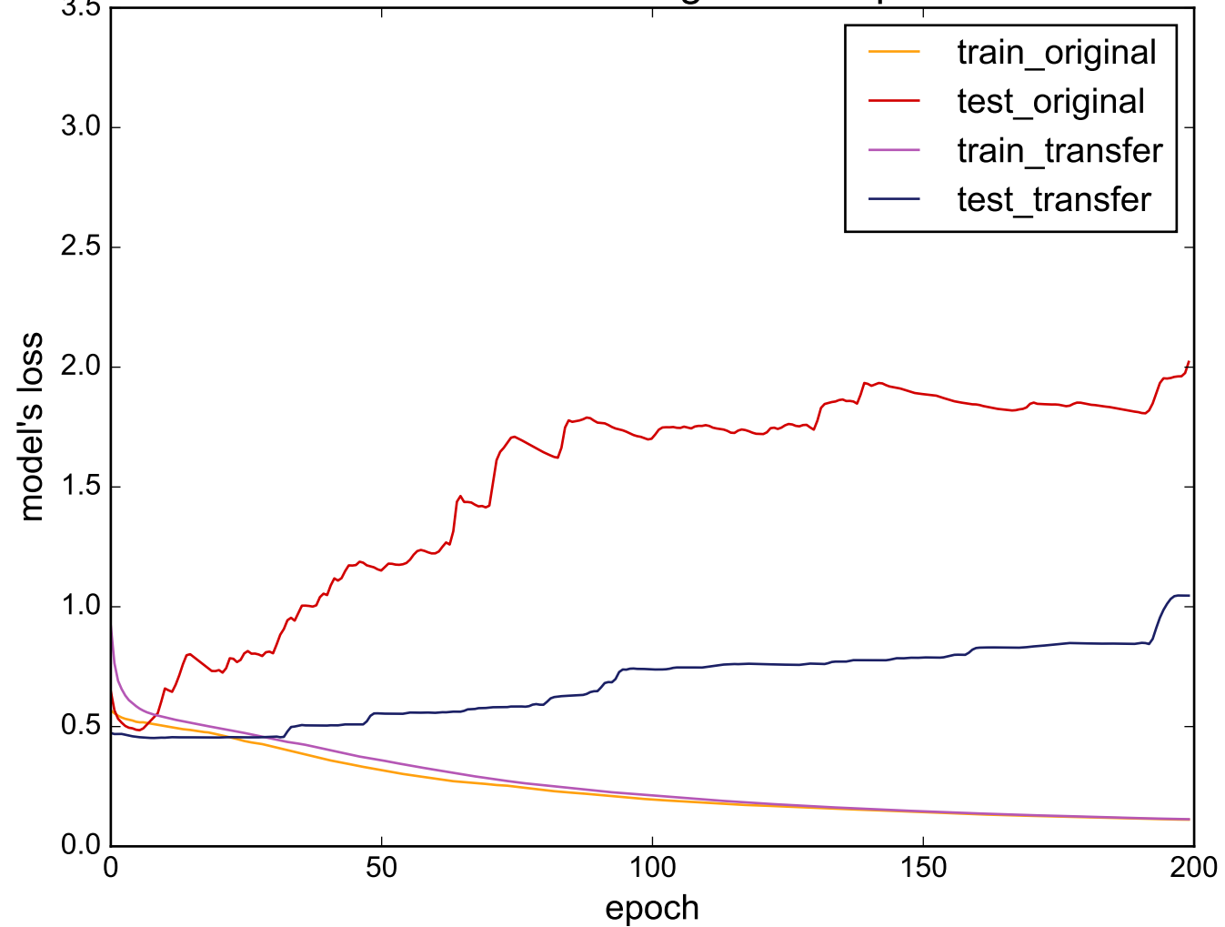
Source: FordB - Target: Earthquakes
