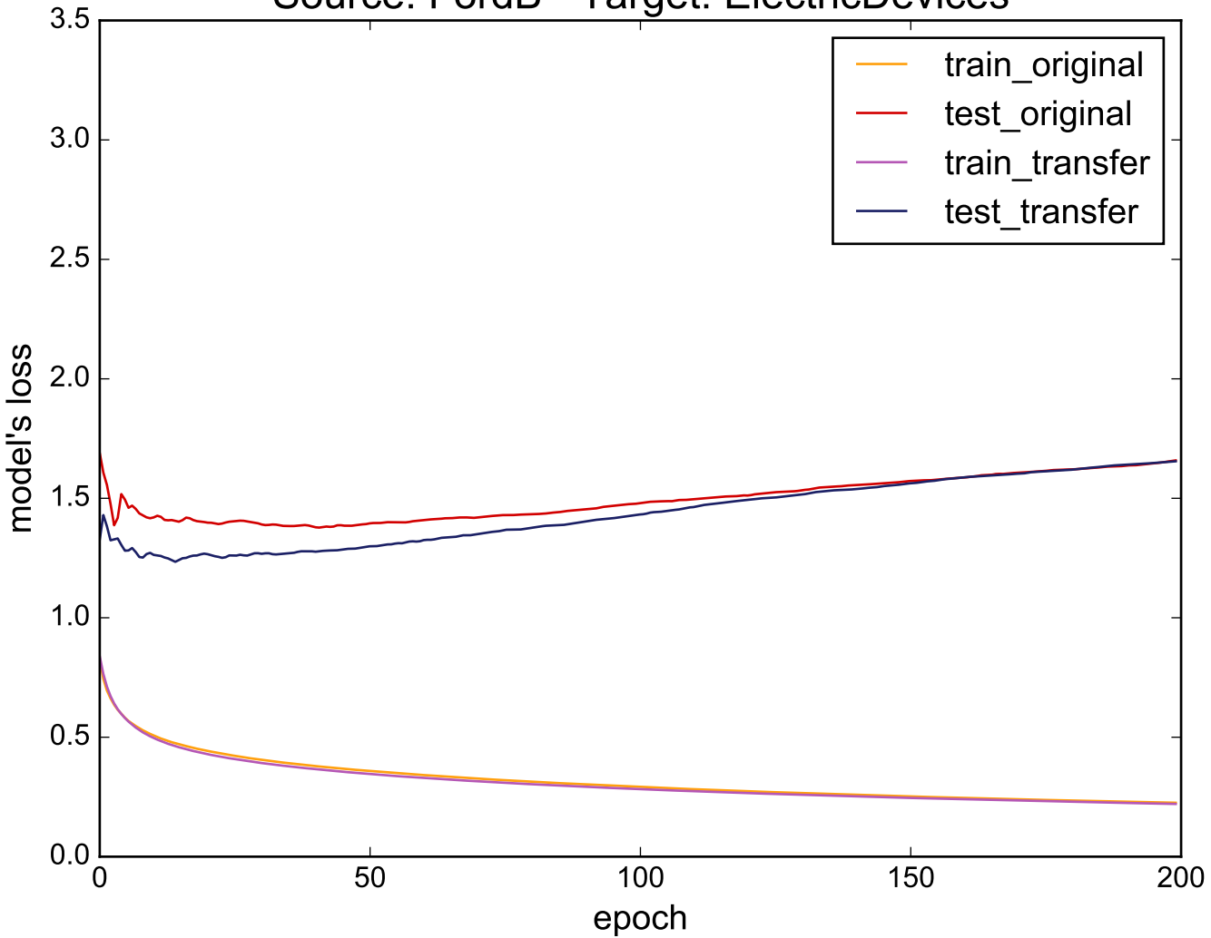
Source: FordB - Target: ElectricDevices
