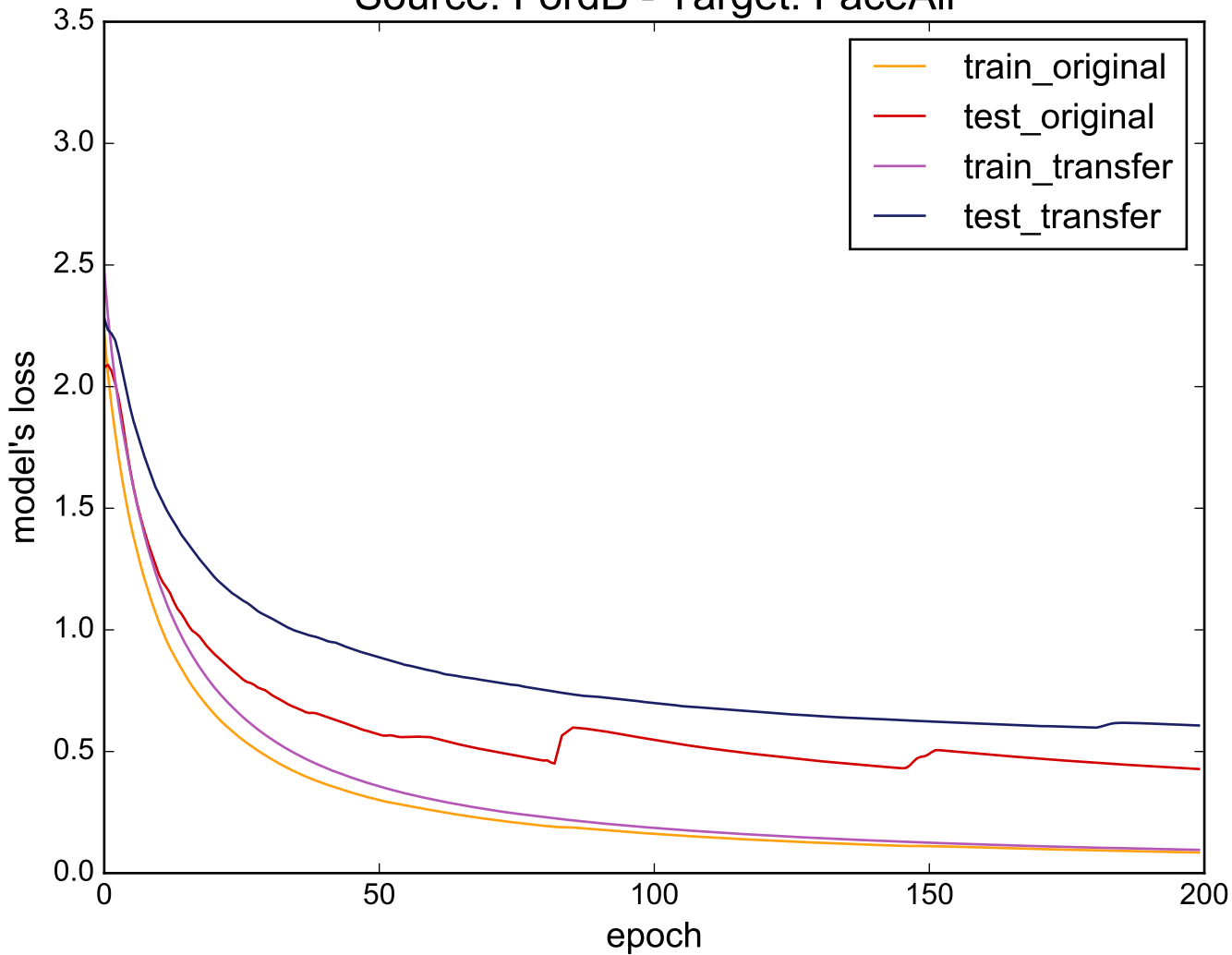
Source: FordB - Target: FaceAll
