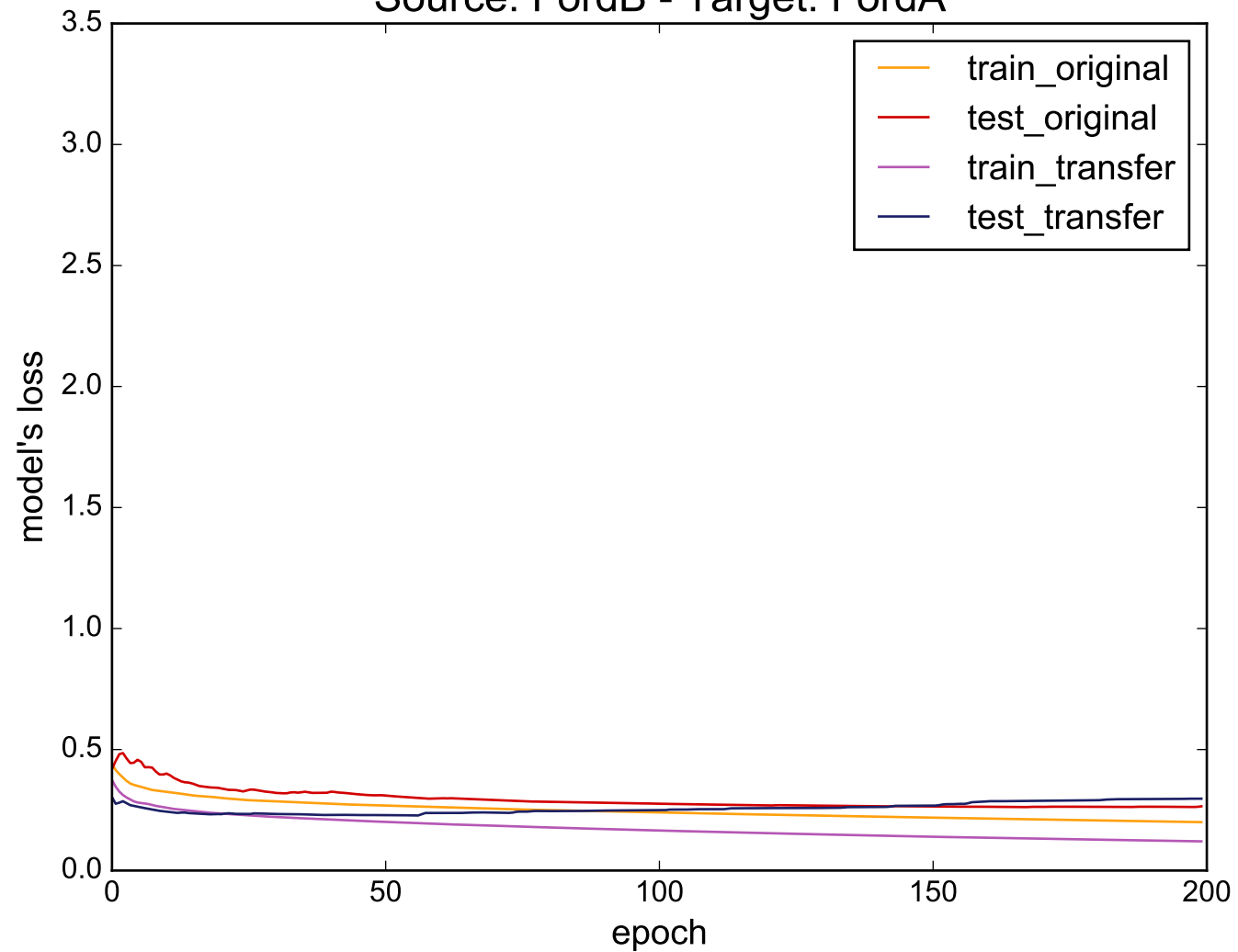
Source: FordB - Target: FordA
