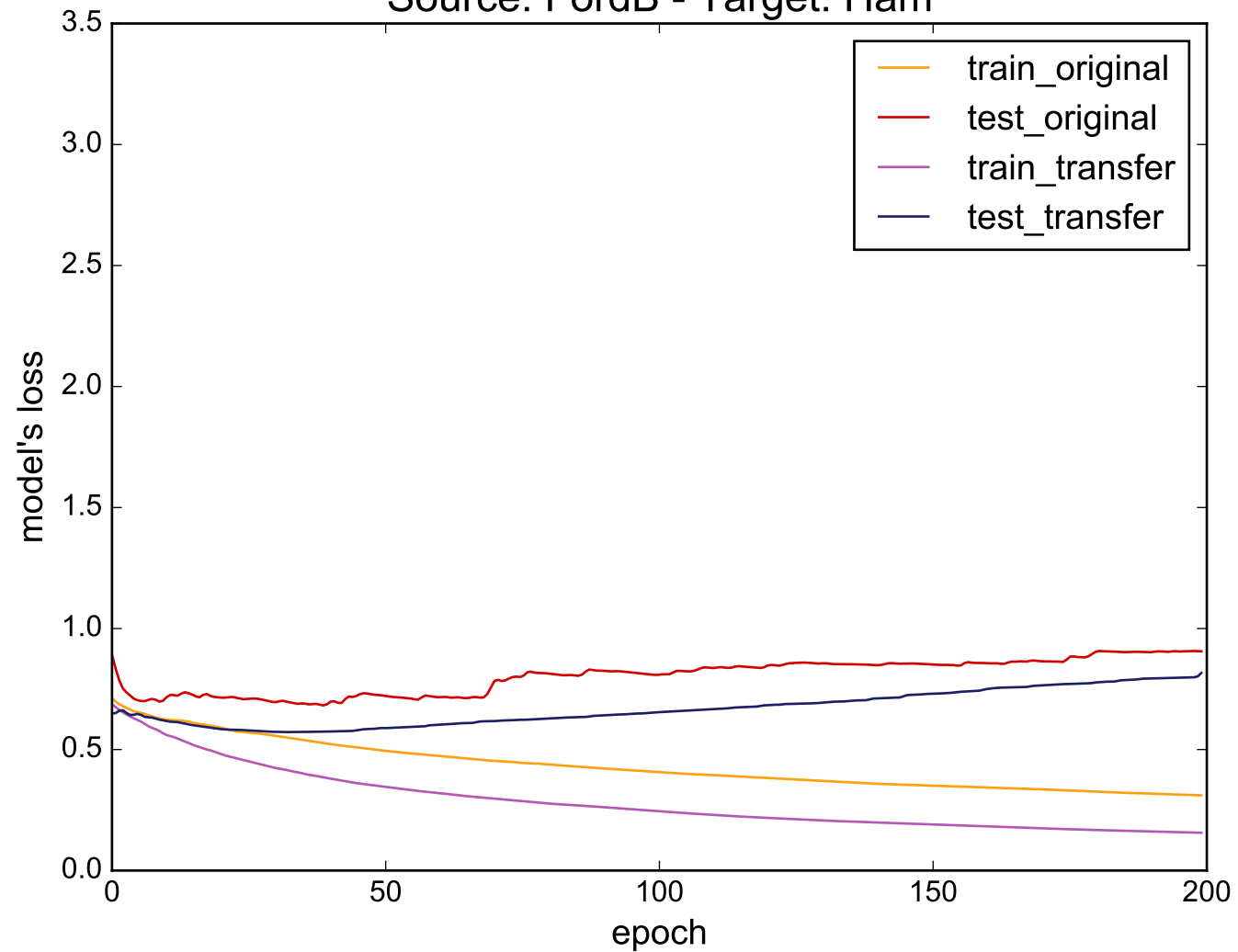
Source: FordB - Target: Ham
