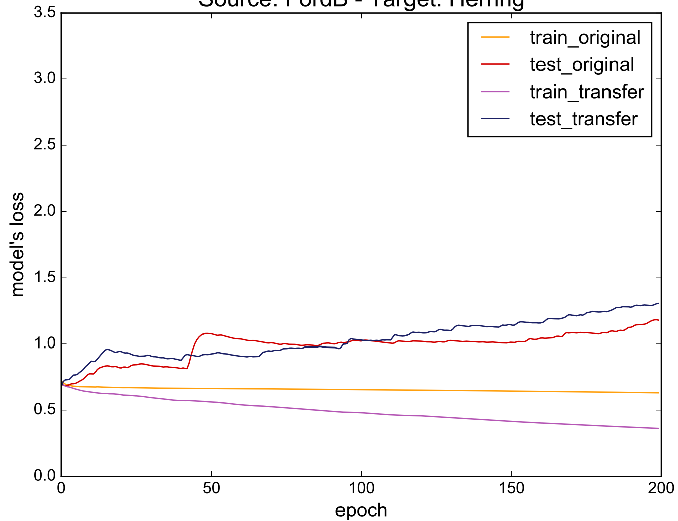
Source: FordB - Target: Herring
