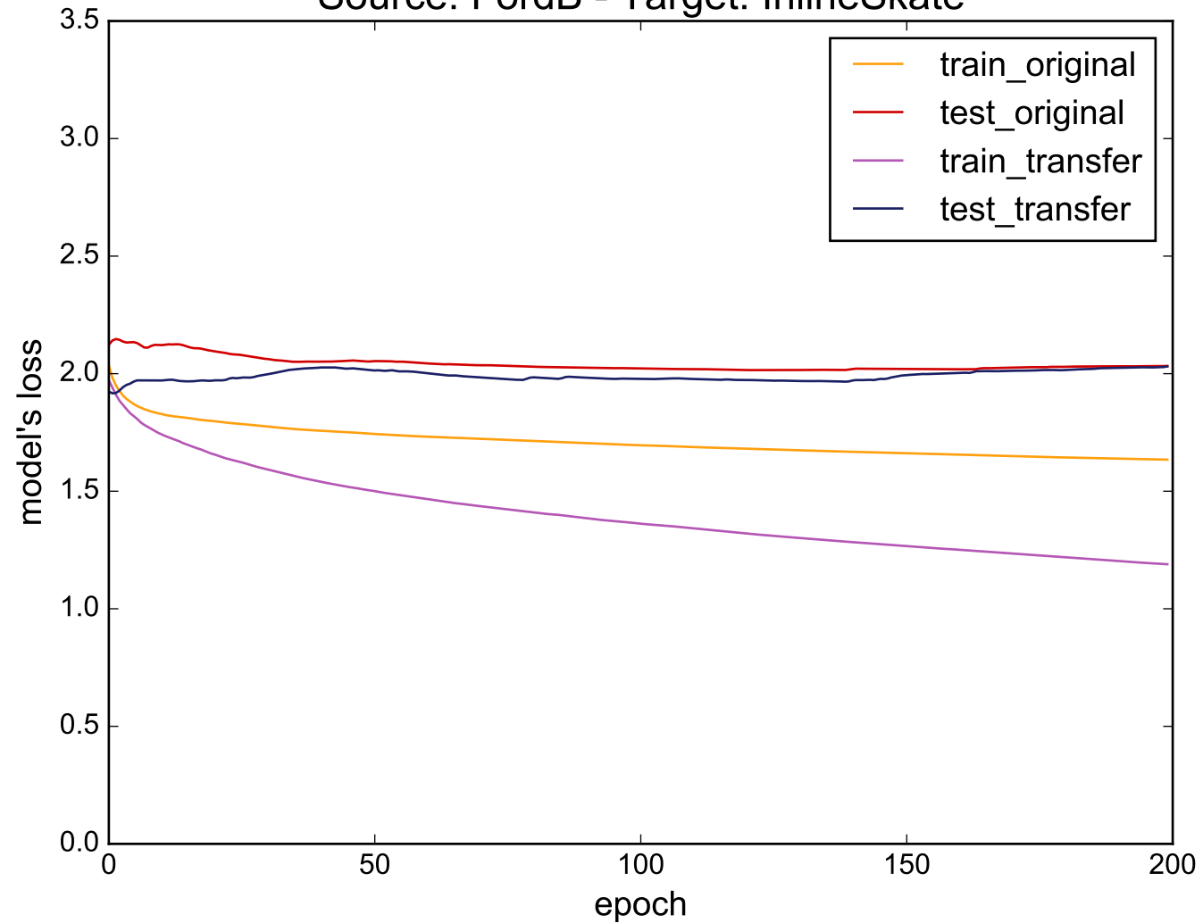
Source: FordB - Target: InlineSkate
