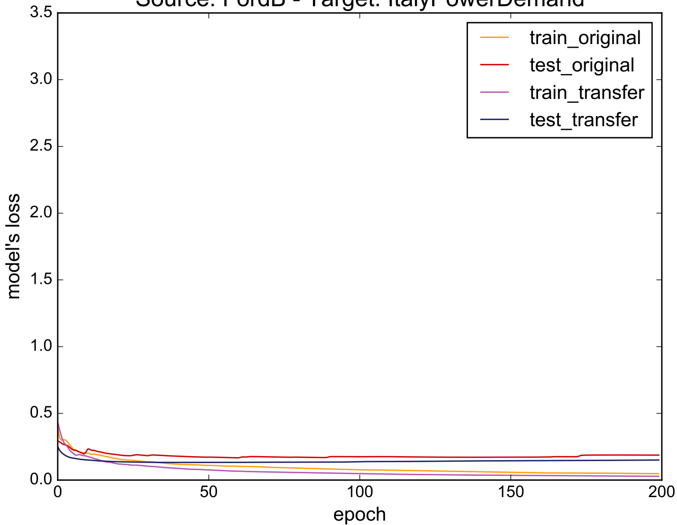
Source: FordB - Target: ItalyPowerDemand
