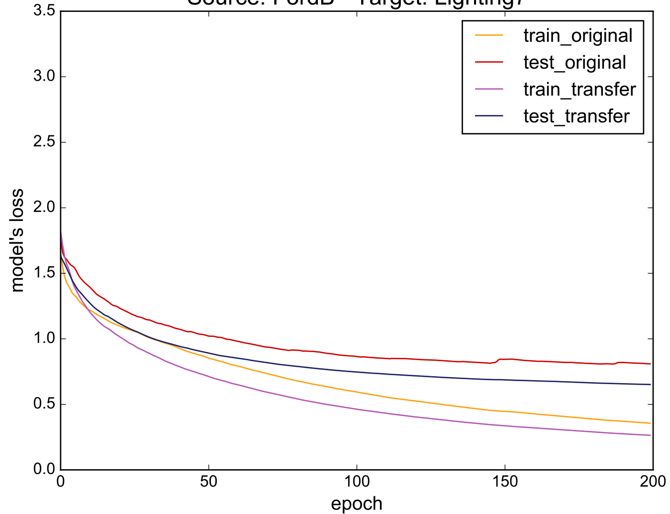
Source: FordB - Target: Lighting7
