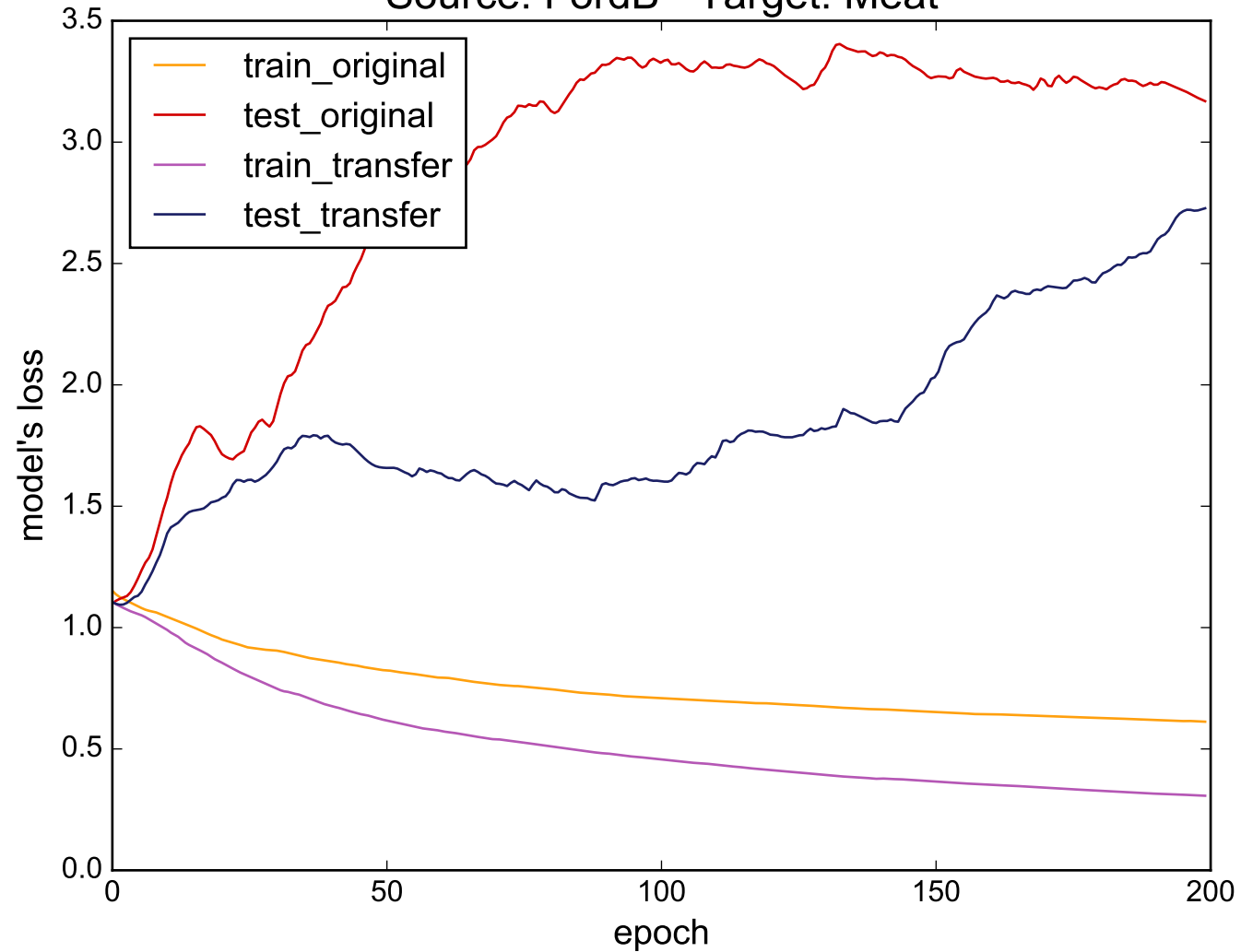
Source: FordB - Target: Meat
