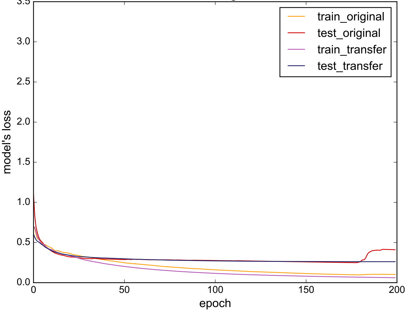
Source: FordB - Target: MoteStrain
