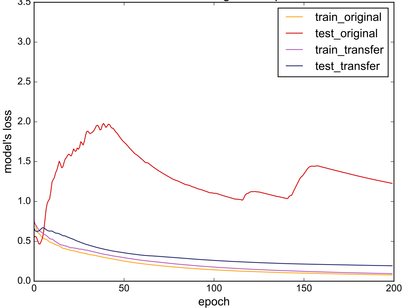
Source: FordB - Target: ShapeletSim
