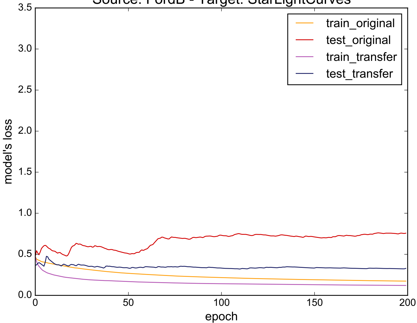
Source: FordB - Target: StarLightCurves
