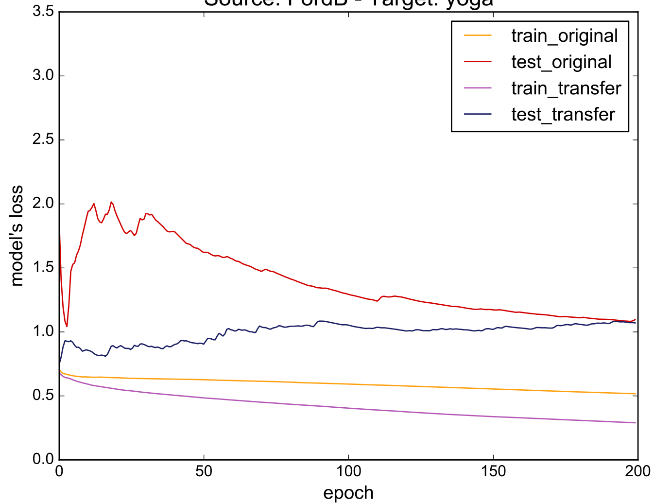
Source: FordB - Target: yoga
