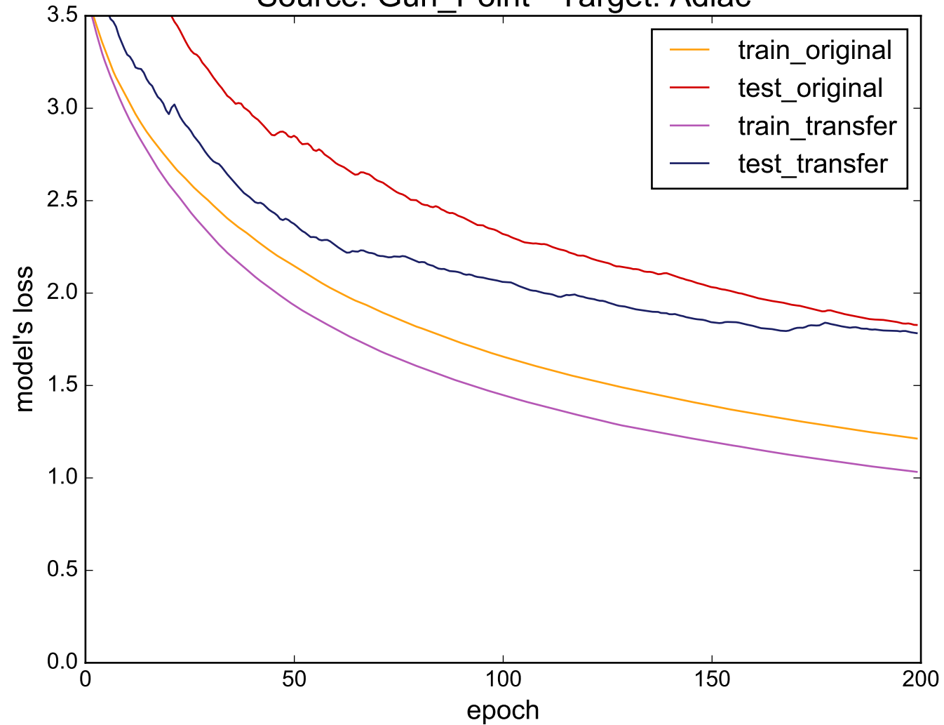
Source: Gun_Point - Target: Adiac
