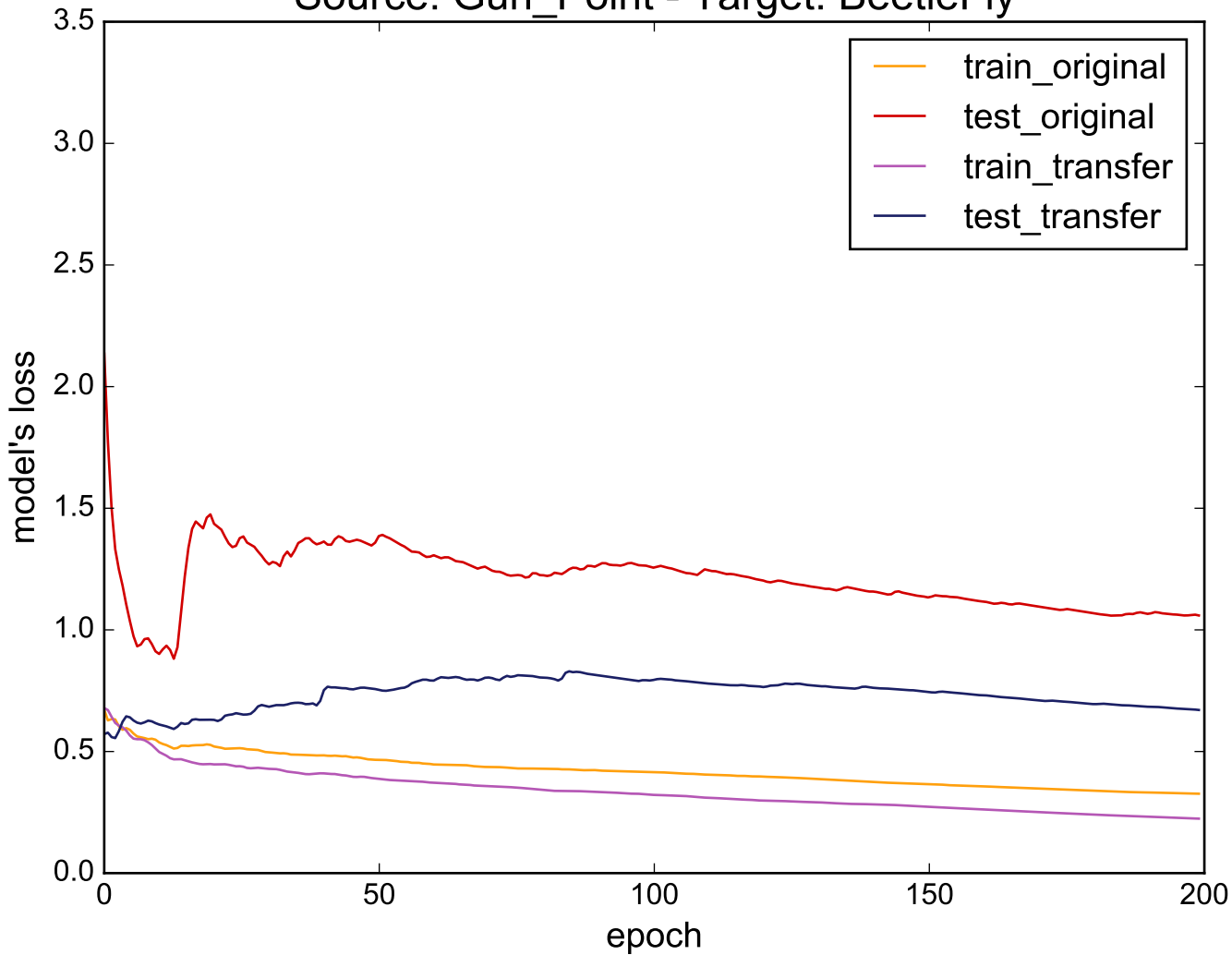
Source: Gun_Point - Target: BeetleFly
