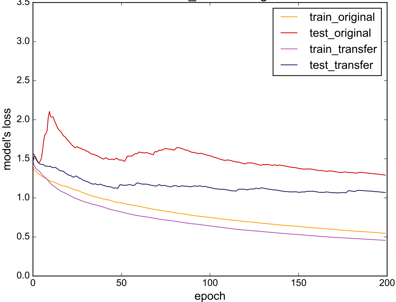
Source: Gun_Point - Target: Car
