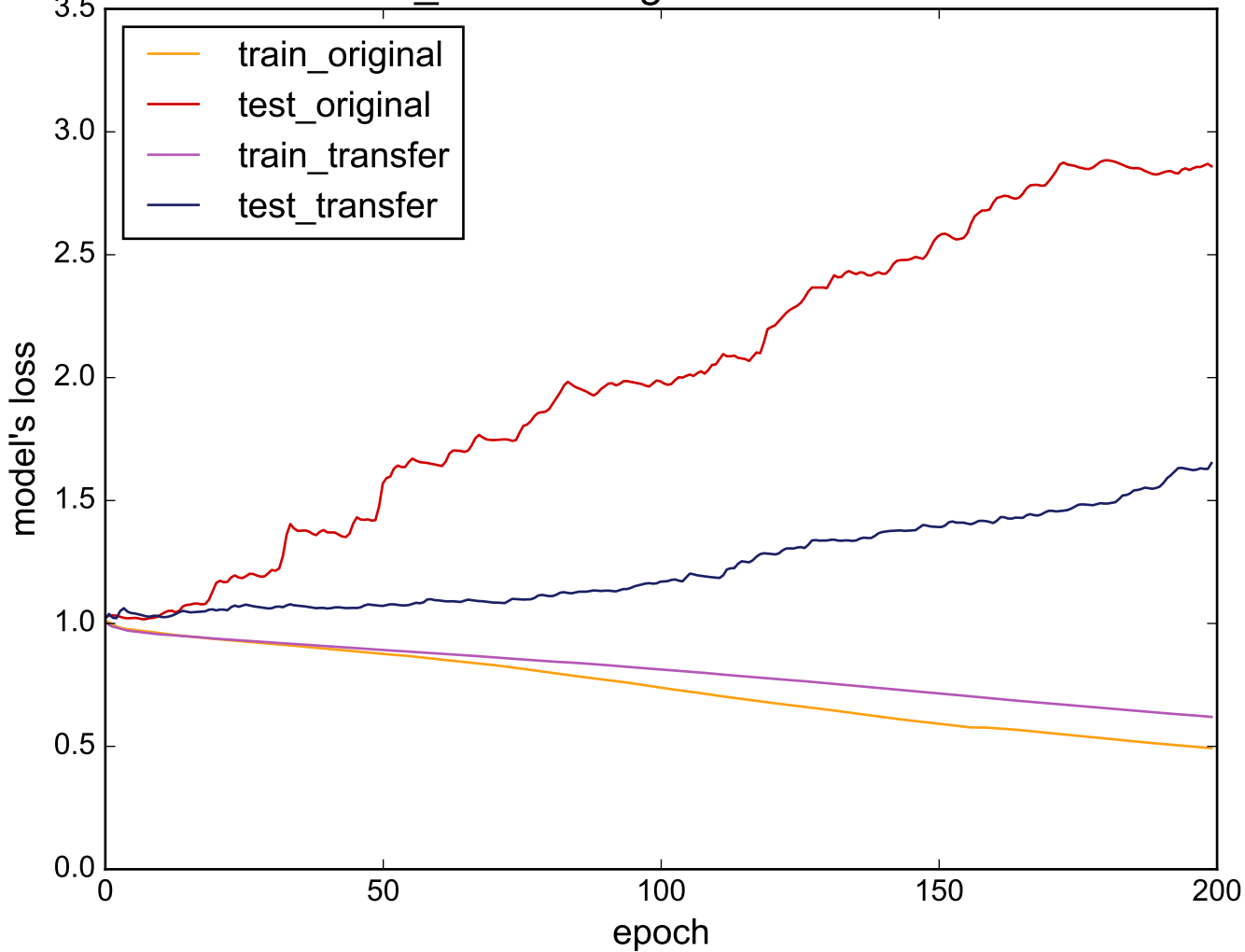
Source: Gun_Point - Target: ChlorineConcentration
