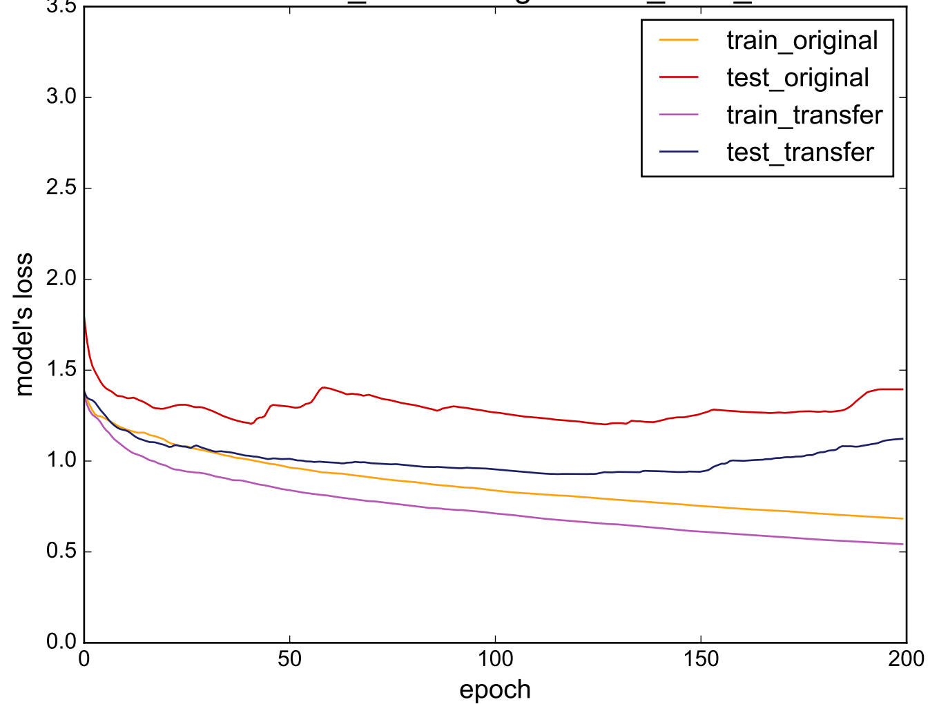
Source: Gun_Point - Target: CinC_ECG_torso
