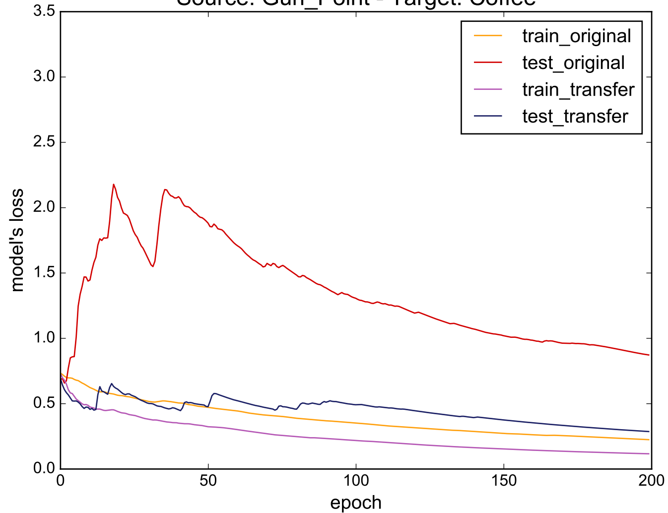
Source: Gun_Point - Target: Coffee
