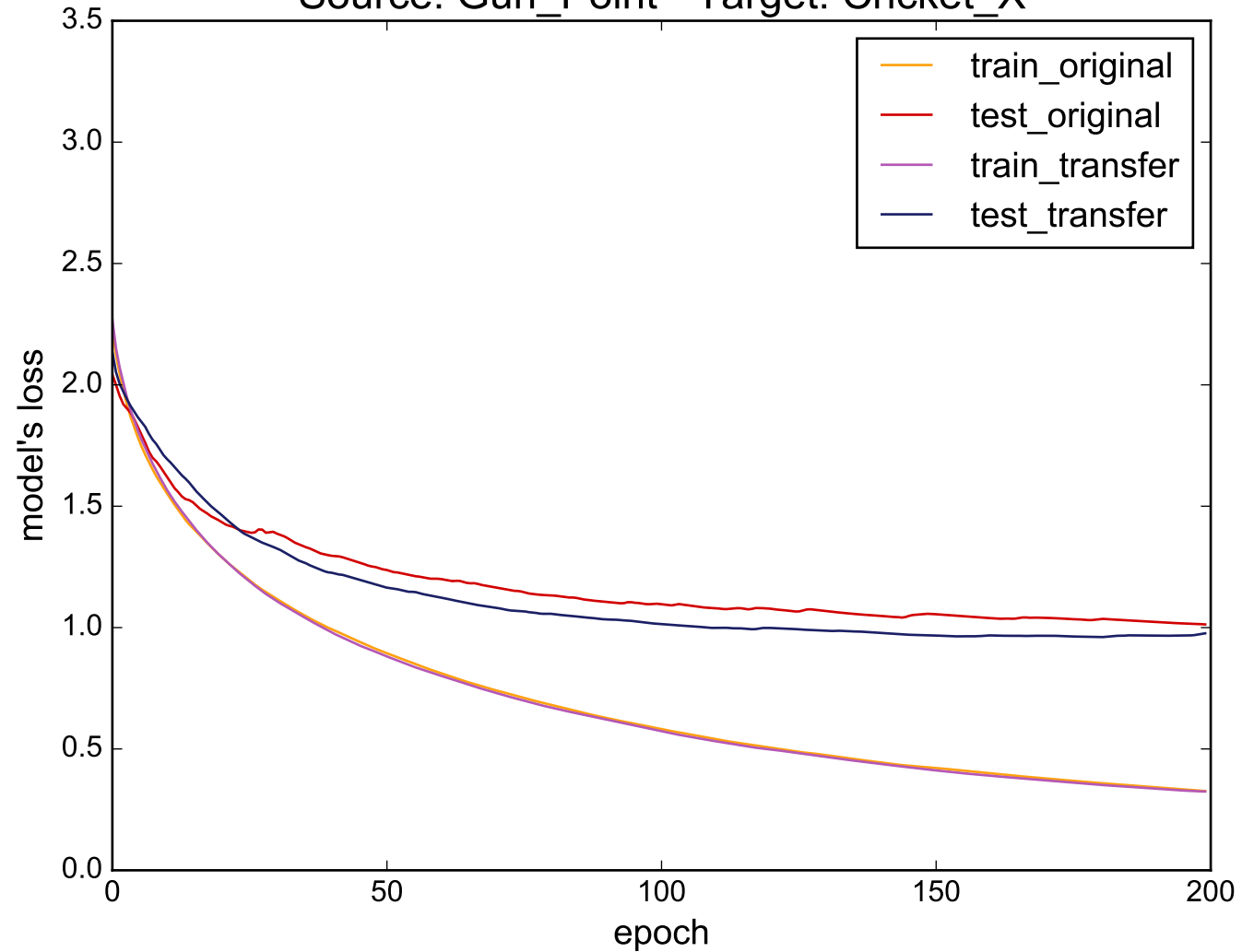
Source: Gun_Point - Target: Cricket_X
